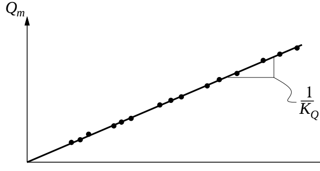
Figure 5: Q_m data versus i - i_o , with curve fit to determine K_Q .
